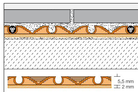
Schlüter®-DITRA-HEAT-DUO
