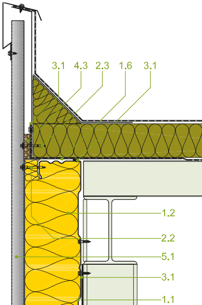
Attika
